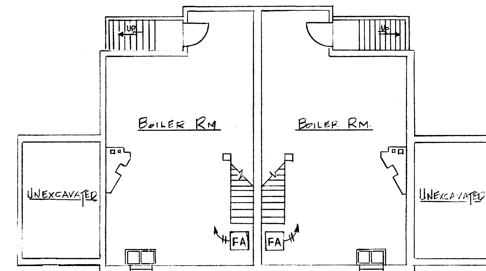
BASEMENT PLAN FLOOR PLAN BLDGS 276, 277, & 278
