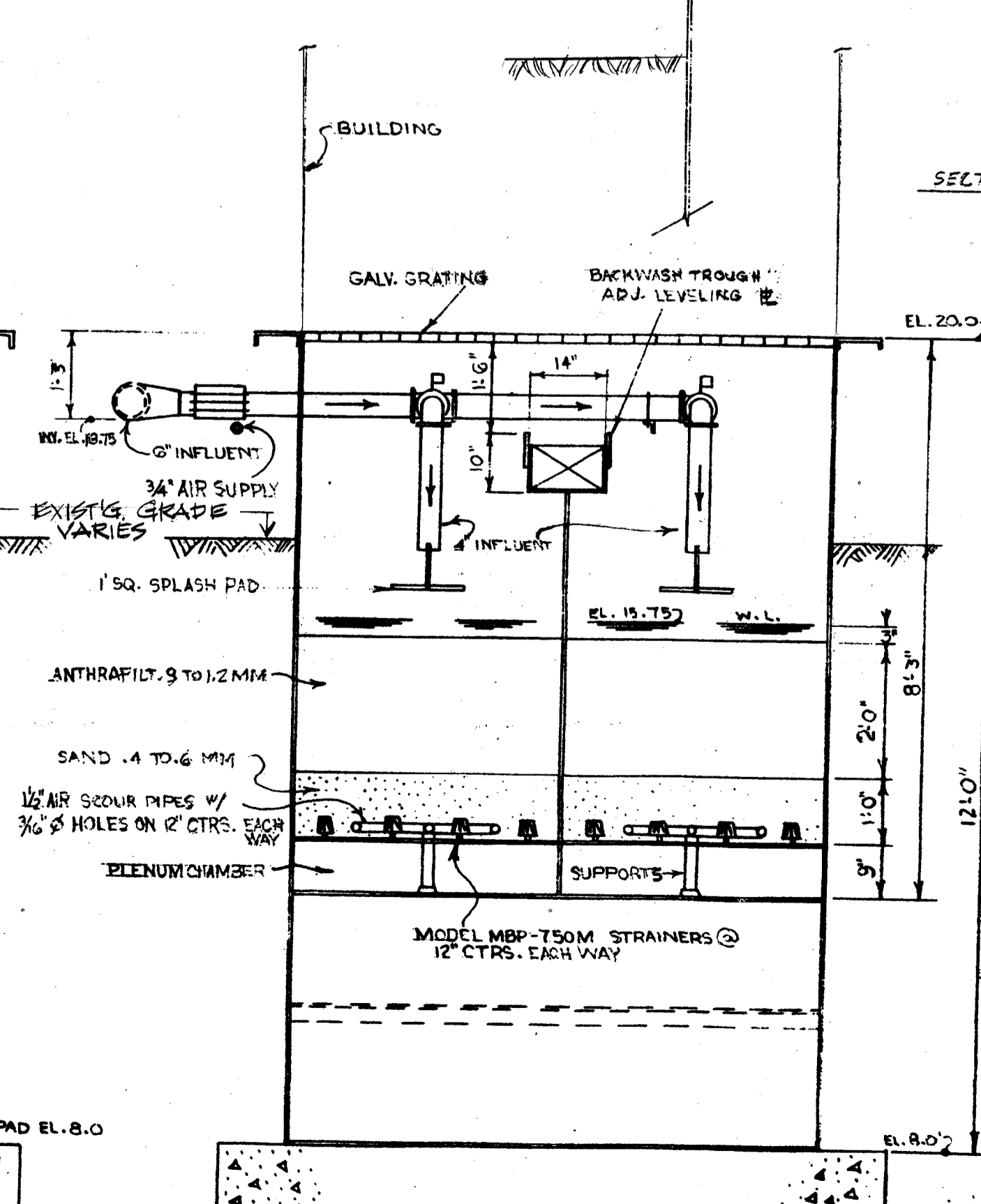
SECTION-CC-
