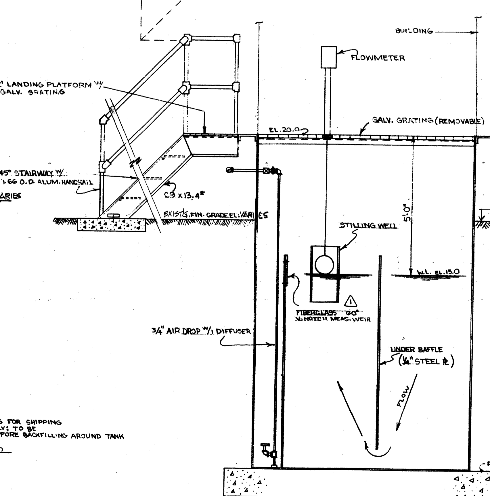
SECTION-BB-
