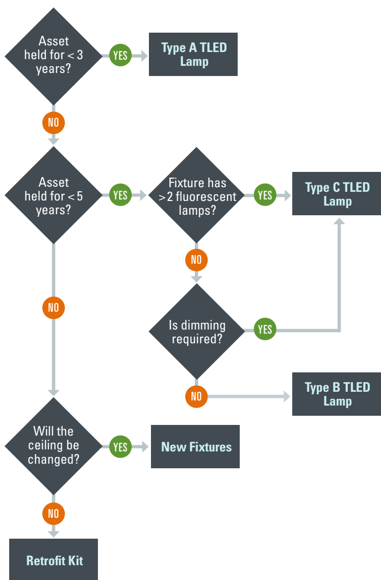
Decision Flowchart for Retrofitting Linear LED Lighting
