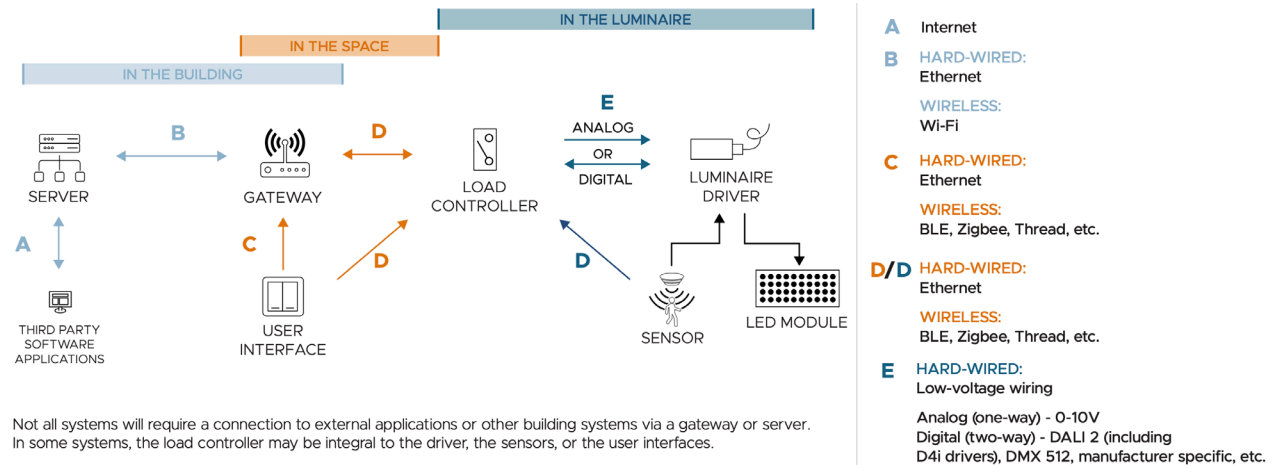
System Architecture with Wiring Controls (Pacific Northwest National Laboratory)
