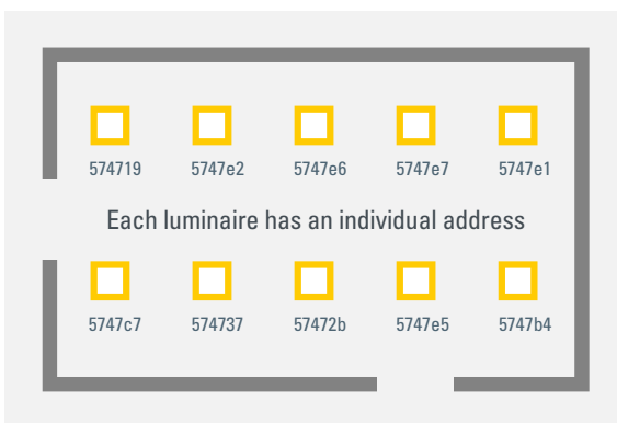
Figure 21 Reflected Ceiling Plan of an Open Office
