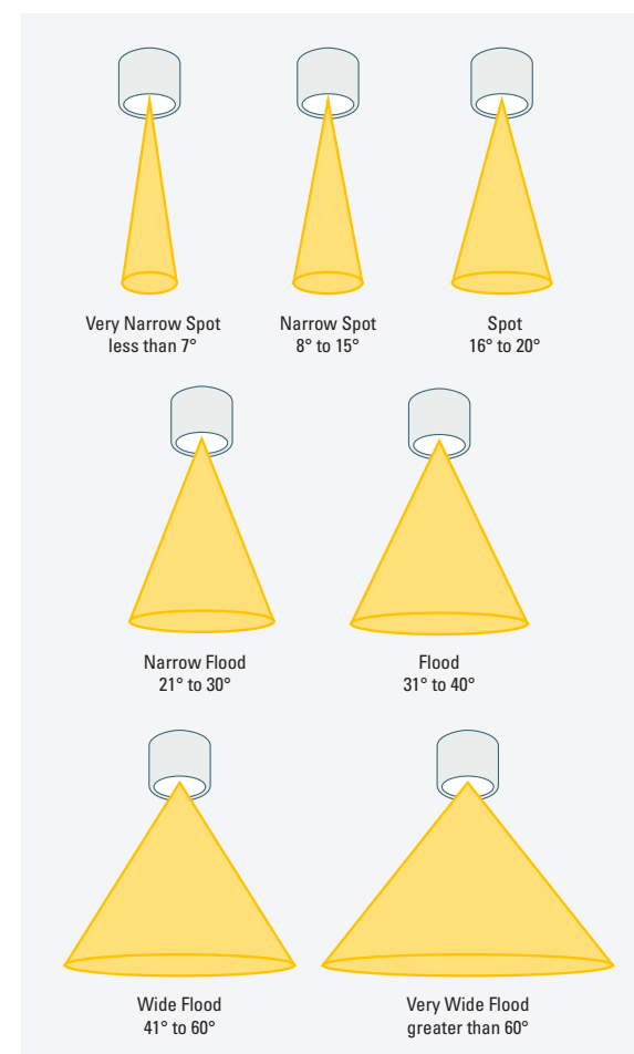
Figure 6 Distribution Can Be Represented by Beam Angles
