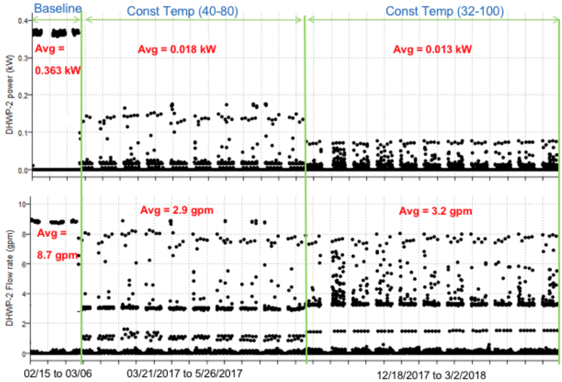
Figure 25 – DHWP-2 Power and Flow
