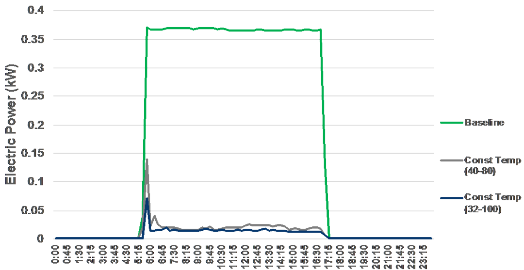
Figure 26 – DHWP-2 Daily Average Electric Power
