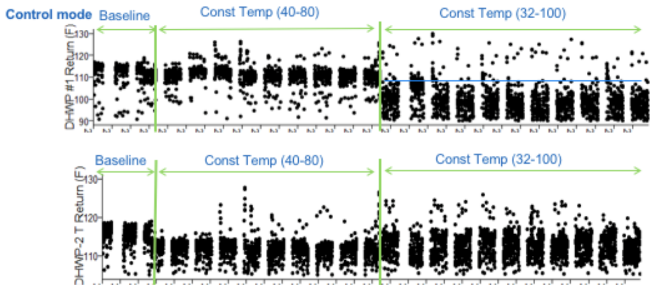
Figure 35 – DHWP-1 and DHWP-2 Return Water Temperature
