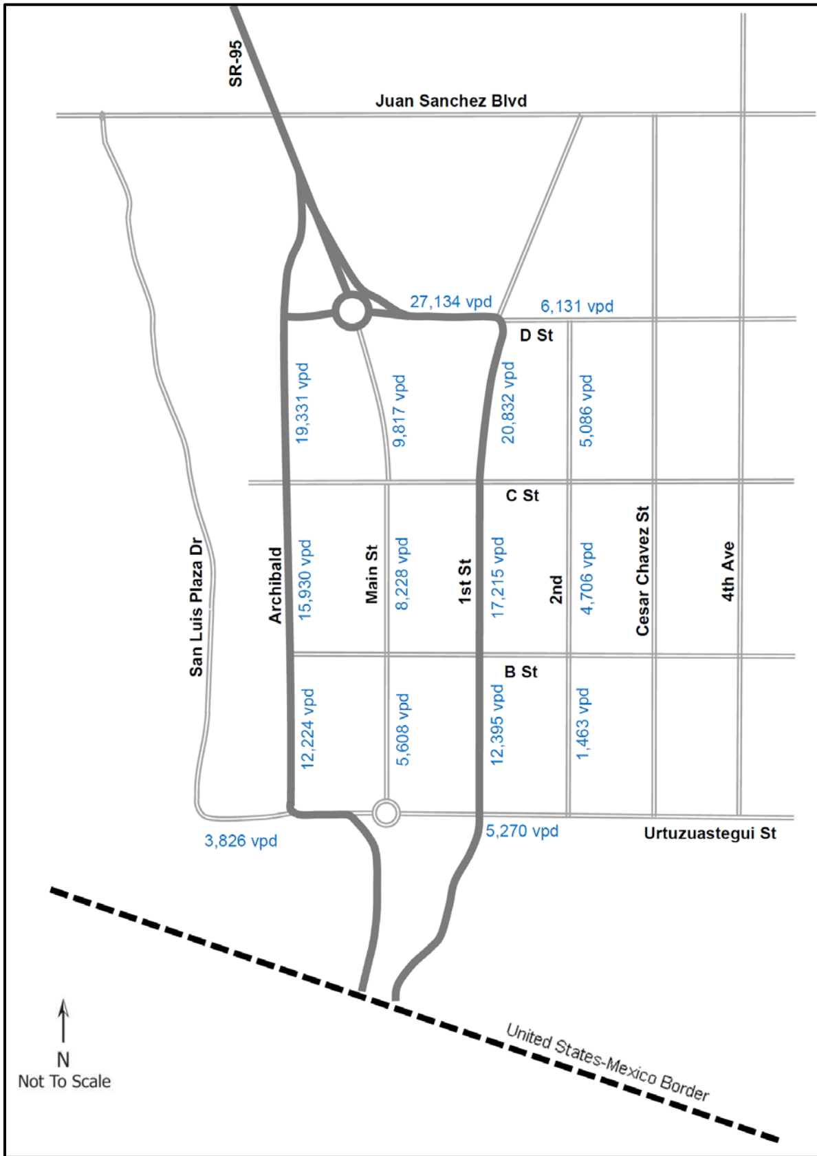
Figure 3-10. Existing Traffic Counts
